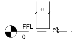
05 Undercut Detail 1 : 5
