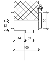
04 Head Detail 1 : 5
